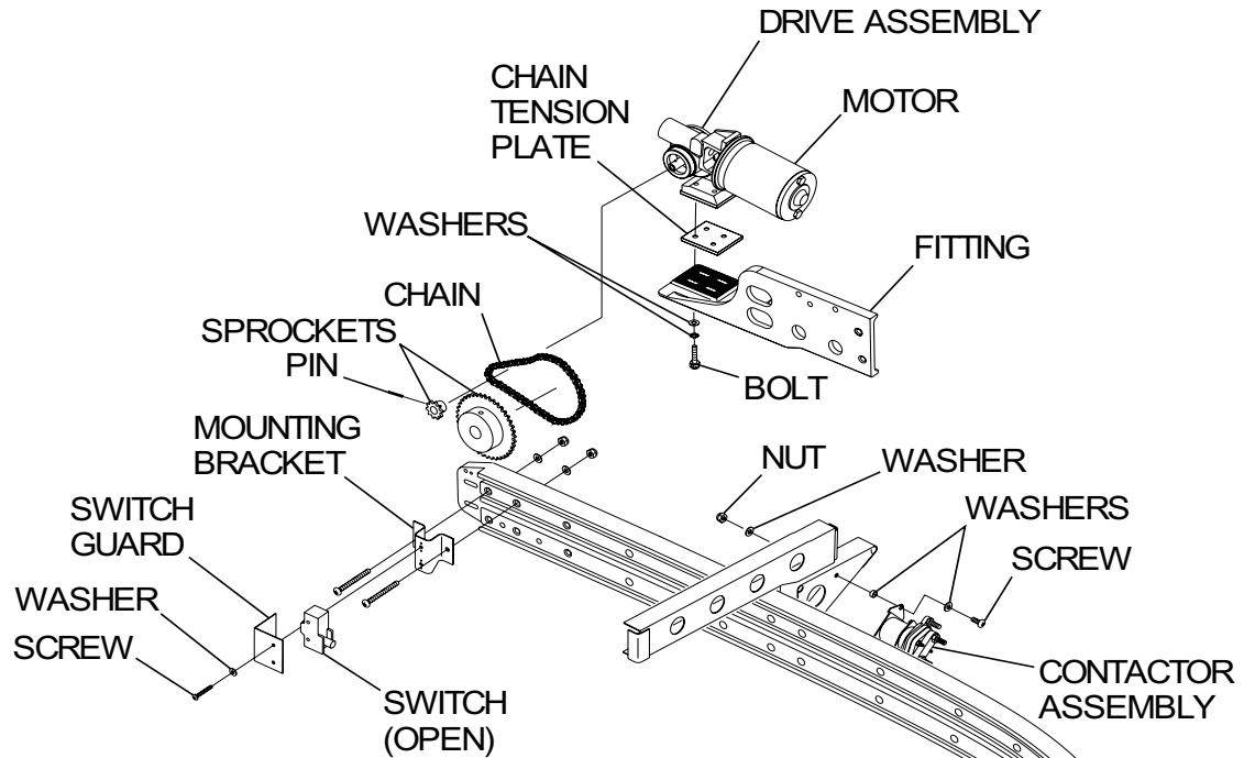
Figure 202 : Sheet 2 : Drive Assembly Installation
