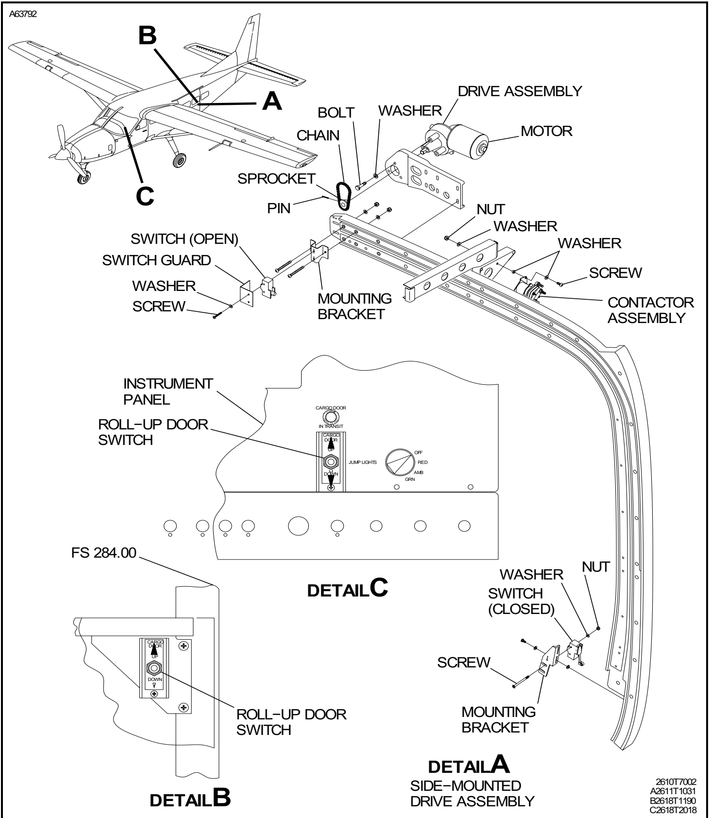
Figure 202 : Sheet 1 : Drive Assembly Installation
