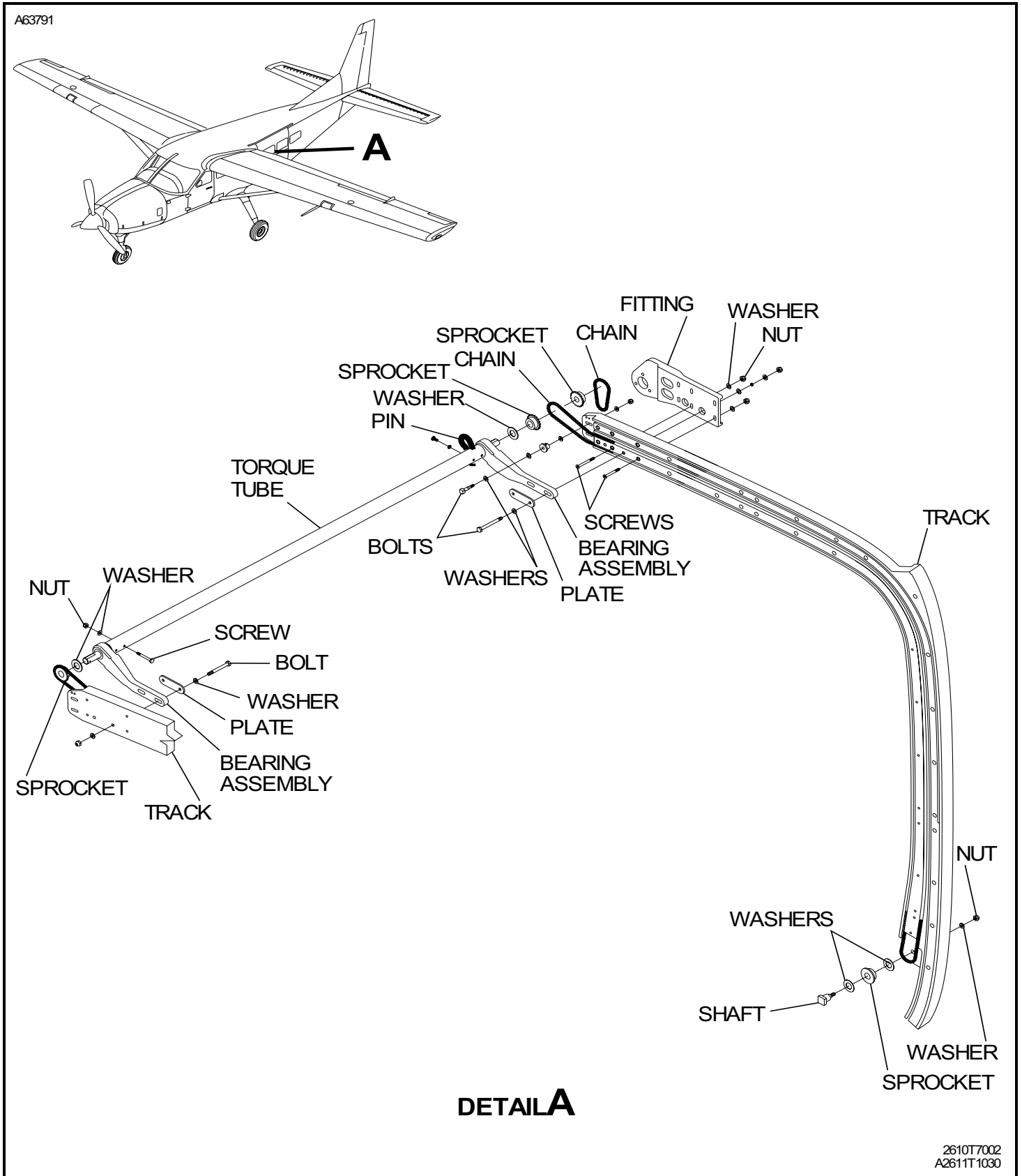
Figure 201 : Sheet 1 : Roll-Up Door Installation
