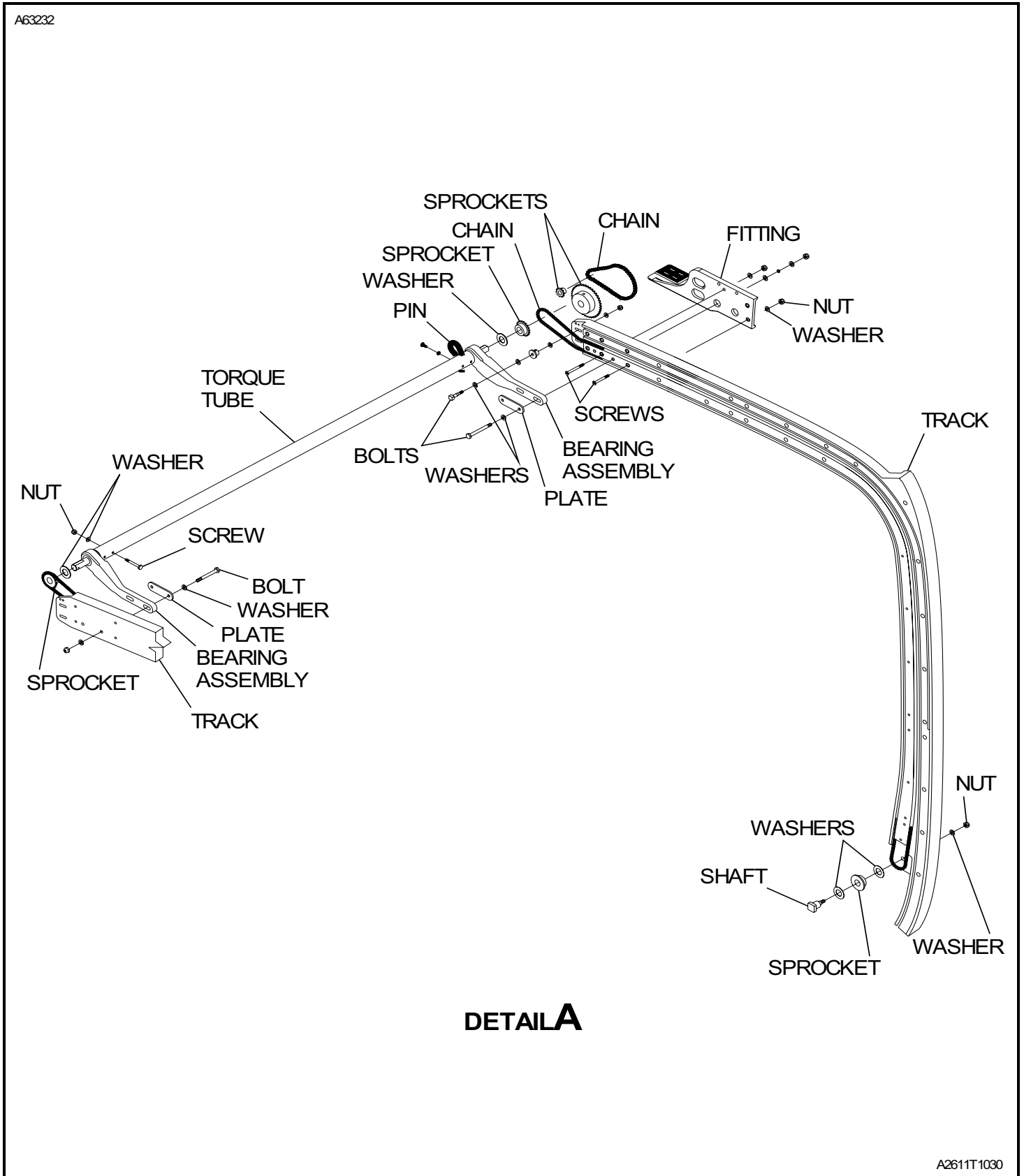
Figure 201 : Sheet 2 : Roll-Up Door Installation
